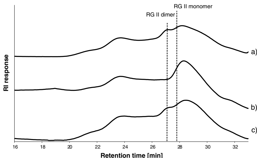
Fig. 1. HPSEC elution patterns of bilberry juice MHR (a) in sodium acetate buffer, pH 3.5, (b) after treatment with 0.1 M HCl dialysed with sodium acetate buffer, pH 3.5, and (c) after treatment with 0.1 M HCl dialysed with sodium acetate buffer, pH 3.5, containing 50 mM boric acid. Vertical lines indicate the elution time of RG II monomer and dimer.
