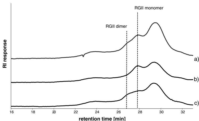
Fig. 2. HPSEC elution patterns of black currant juice MHR in (a) sodium acetate buffer, pH 3.5, (b) after treatment with 0.1 M HCl followed by dialysis against sodium acetate buffer pH 3.5, and (c) after treatment with 0.1 M HCl followed by dialysis against sodium acetate buffer, pH 3.5, containing 50 mM boric acid. Vertical lines indicate the elution time of RG II monomer and dimer.
